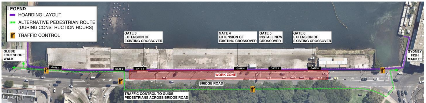
Figure 1: Gate modification and vehicular crossover works location
